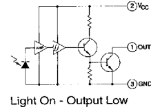
OPL801-OC (Open-Collector Output) Inverter
