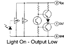
OPL801-OC (Open-Collector Output) Inverter
