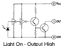
OPL800-OC (Open-Collector Output) Buffer
